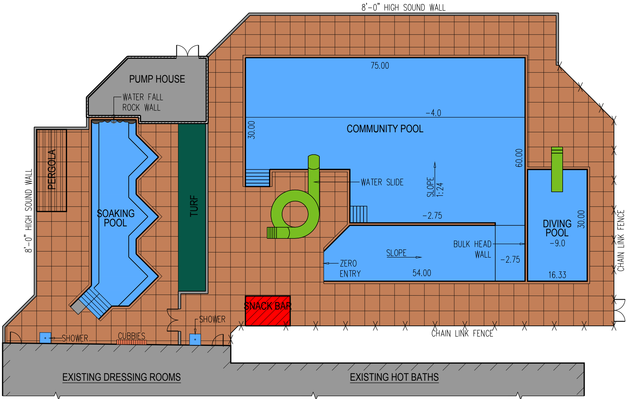
PROPOSED SALIDA OUTDOOR POOLS PLAN
